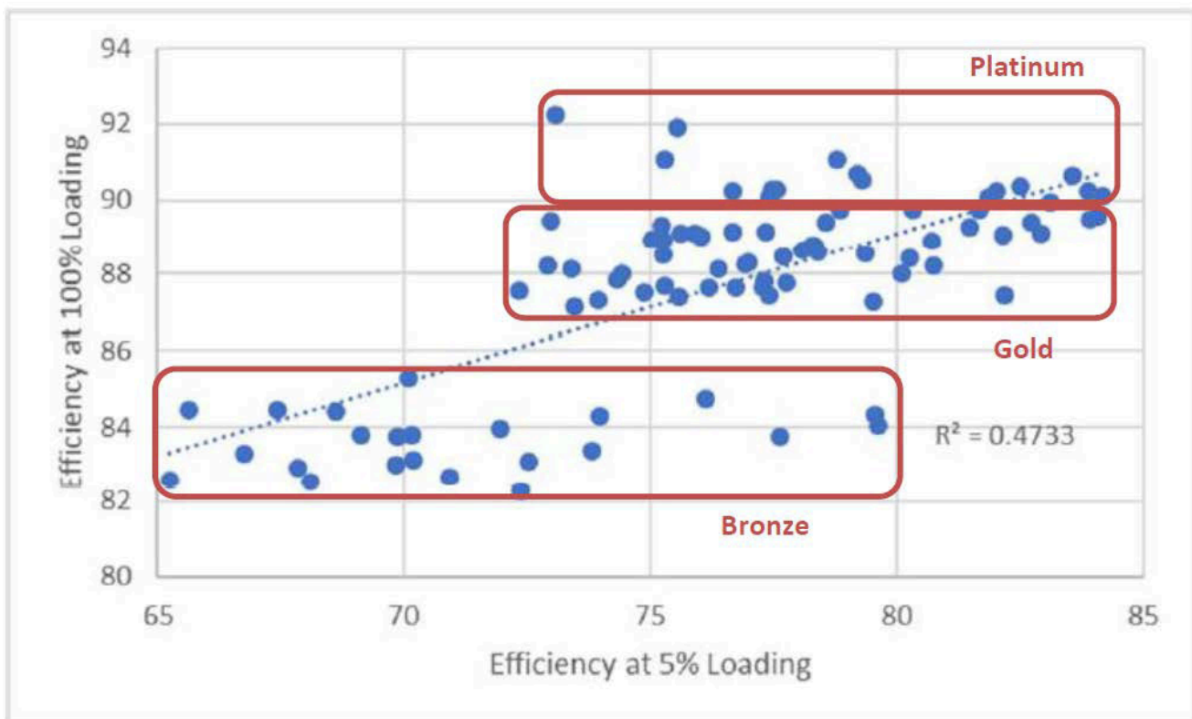
Figure 3. Efficiency at 5% Loading versus Efficiency at 100% Loading.
